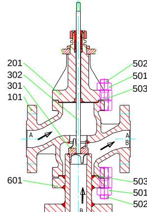
MV 5221, PV 6221 DN 25 – 50, PN 63 – 100
