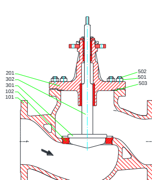
MV 54112, PV 64112 2 DN 250 – 400, PN 16 – 40
