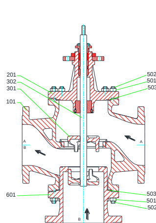
MV 5431, PV 6431 DN 80 – 250, PN 63 – 100
