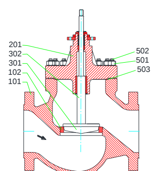
MV 54112, PV 64112 2 DN 250 – 300 2 , PN 63 – 100
