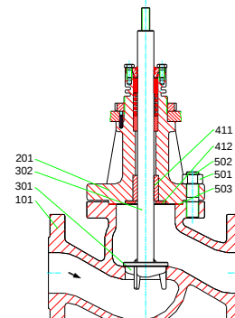
MV 54111, PV 64111 1 DN 40 – 300 1 , PN 63 – 160 3
